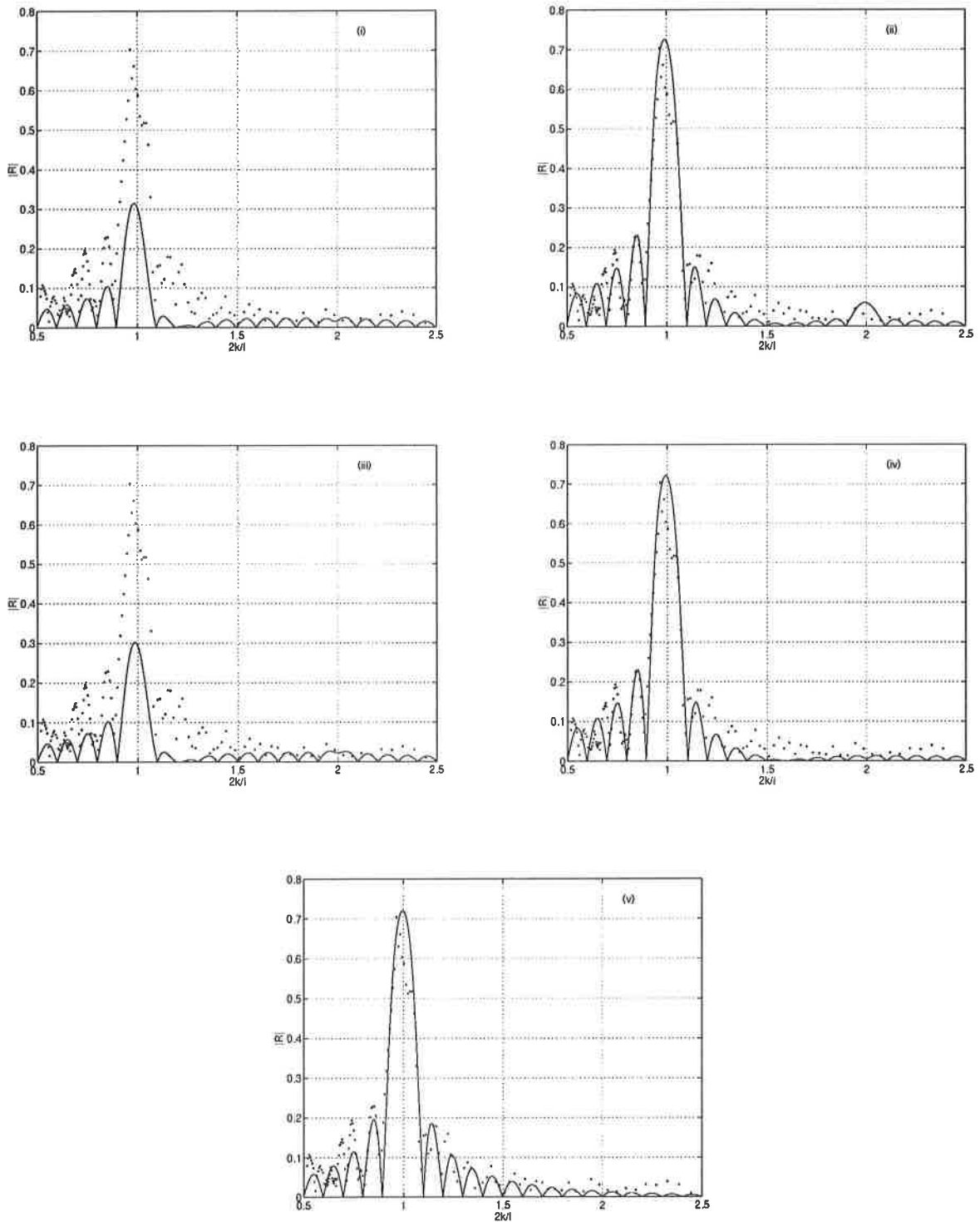
Figure 3: Comparison of computed reflection coefficients for single sinusoidal ripple with n = 10 and d/h_0 = 0.16 .
