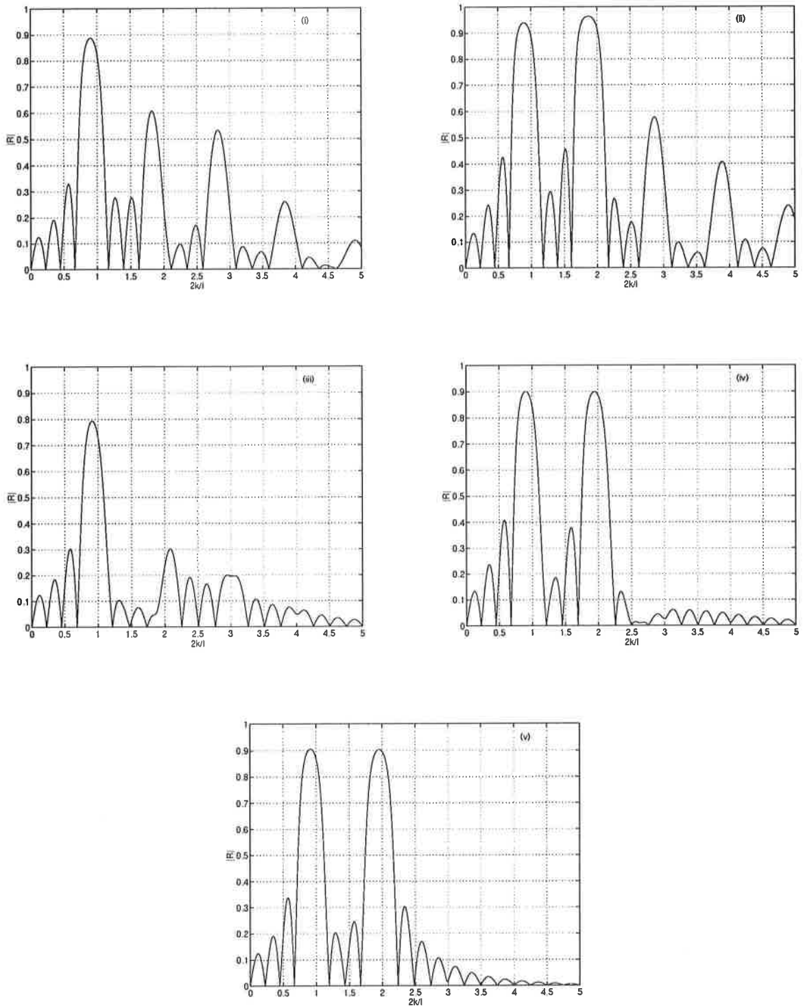
Figure 5: Comparison of computed reflection coefficients for doubly sinusoidal ripple with n = 4 , m = 2 and d/h_0 = 0.4 .
