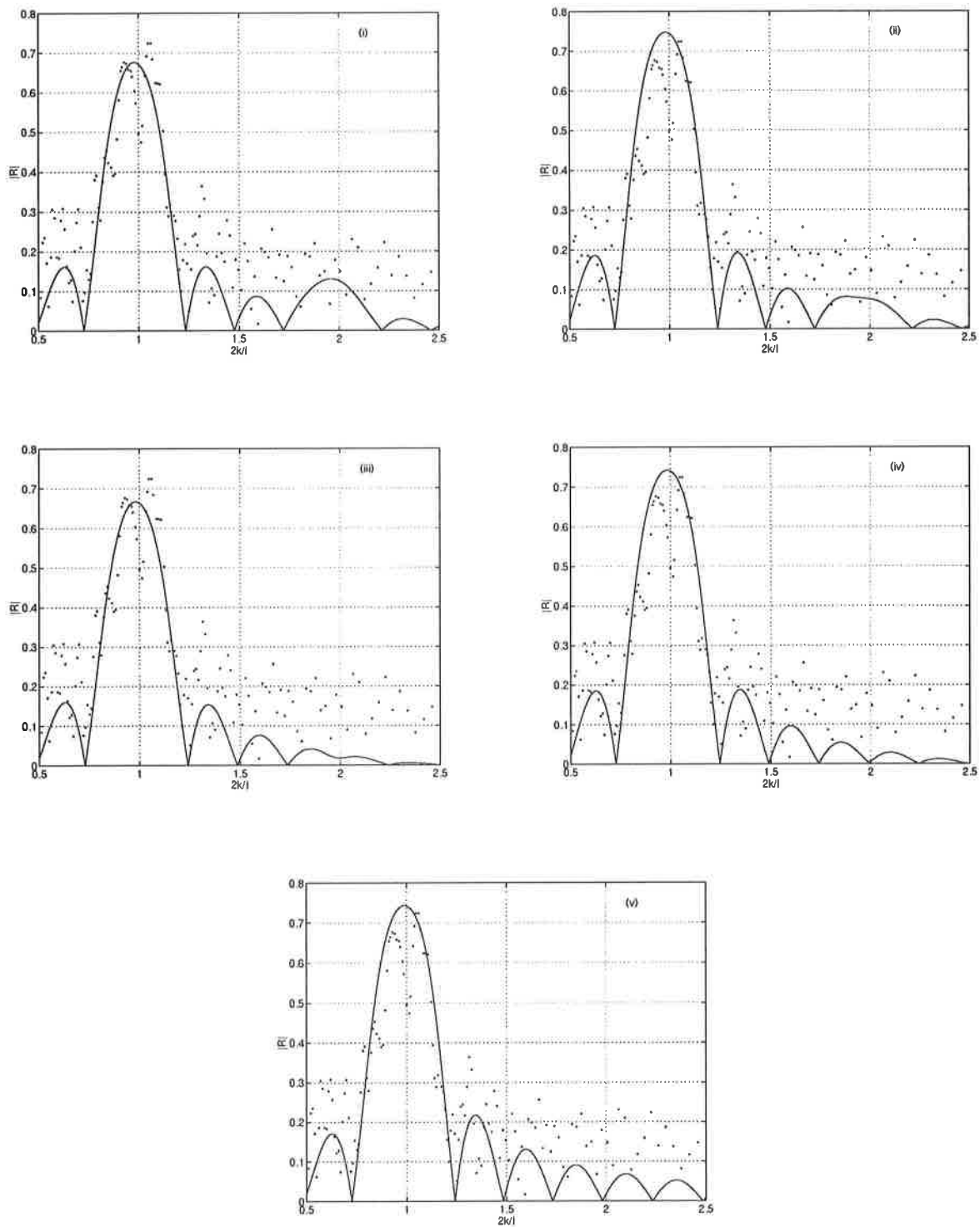
Figure 2: Comparison of computed reflection coefficients for single sinusoidal ripple with n = 4 and d/h_0 = 0.32 .
