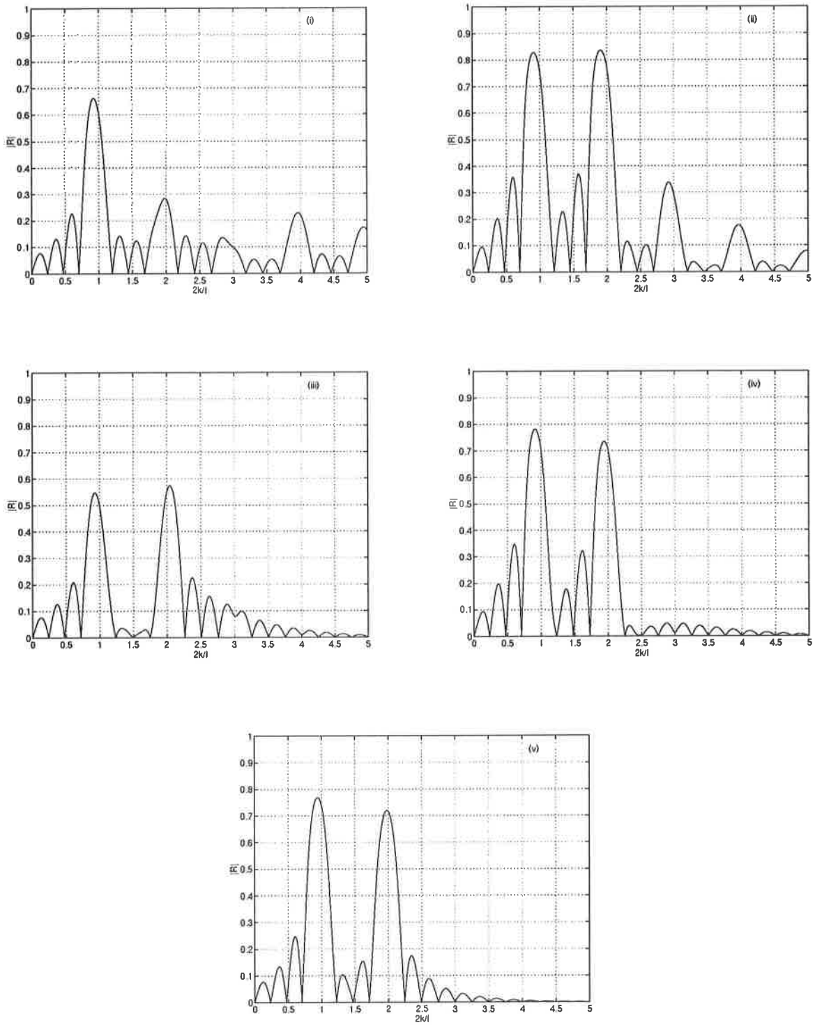
Figure 4: Comparison of computed reflection coefficients for doubly sinusoidal ripple with n = 4 , m = 2 and d/h_0 = 0.33 .
